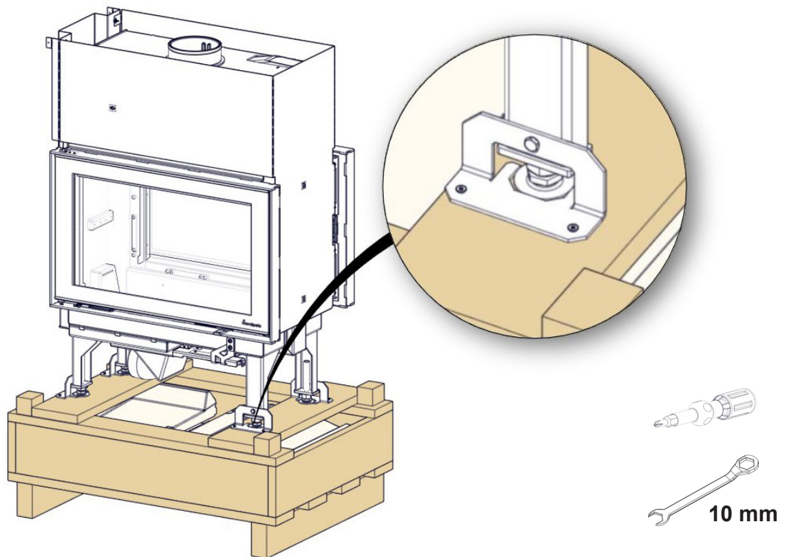
FIG 2 Removing the insert from the pallet
