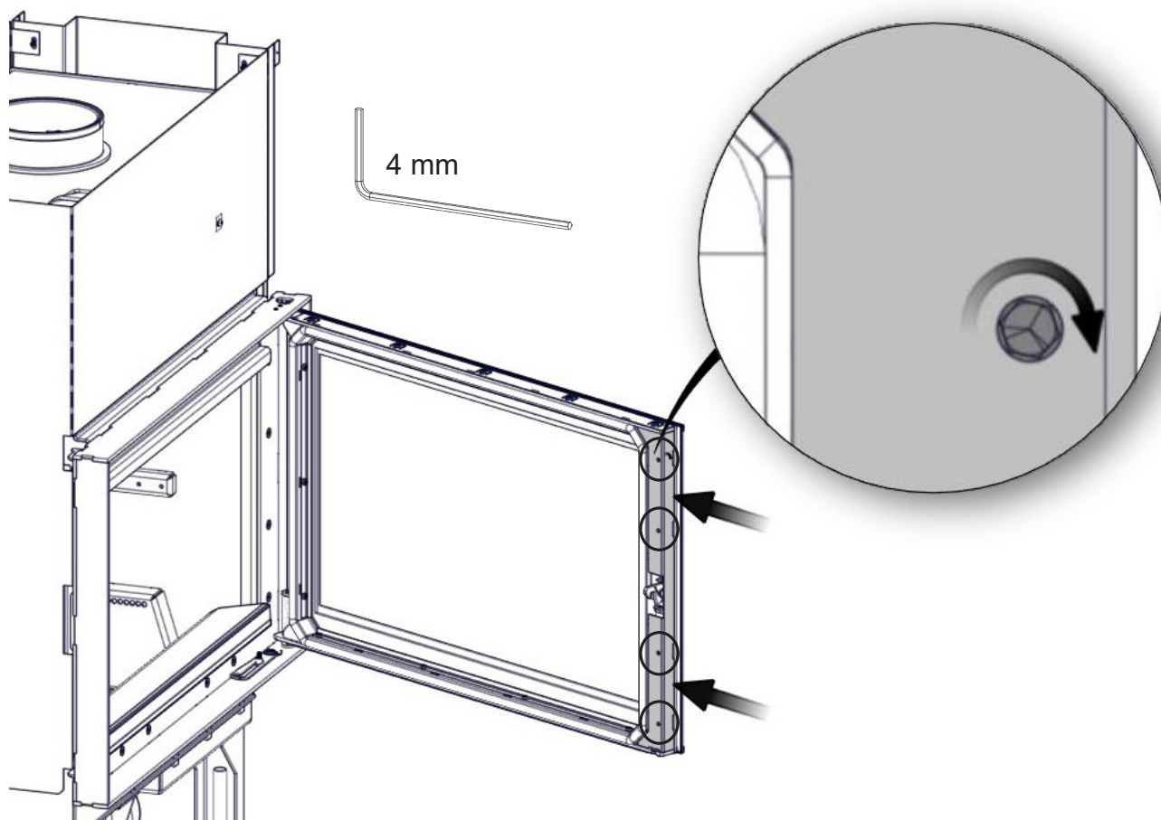
FIG 5 f Right door handle assembling
