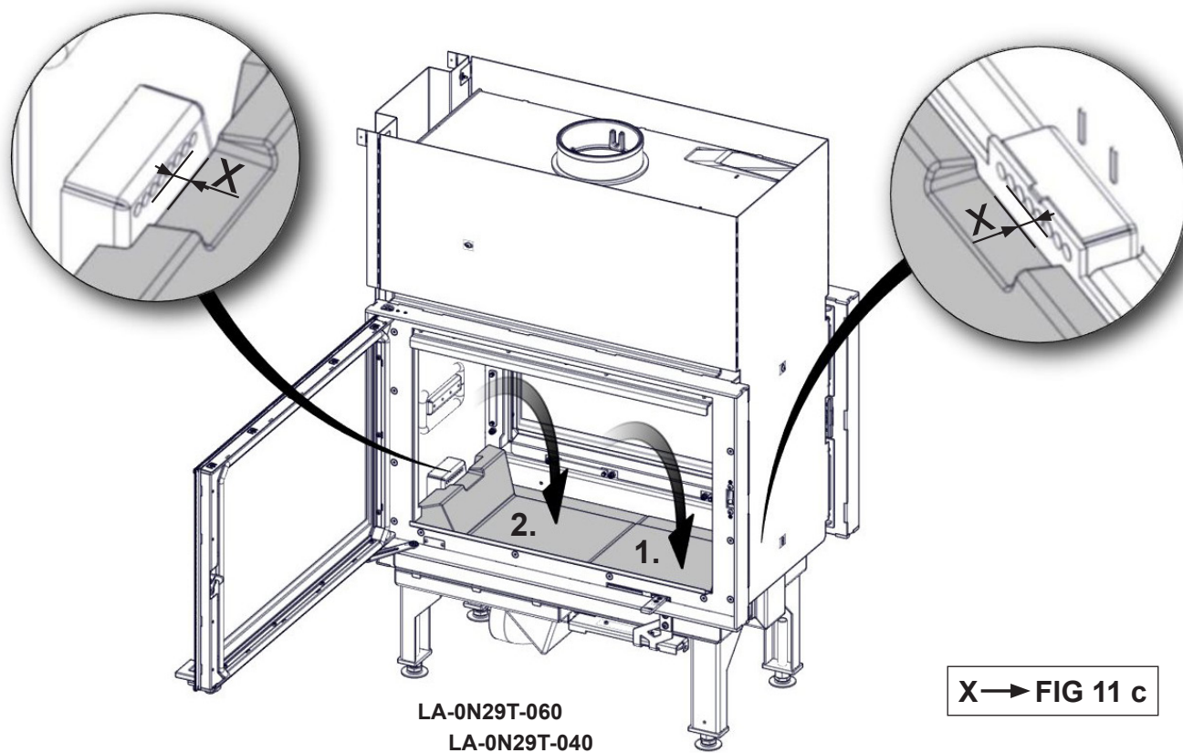
FIG 11 Thermotte assembling
